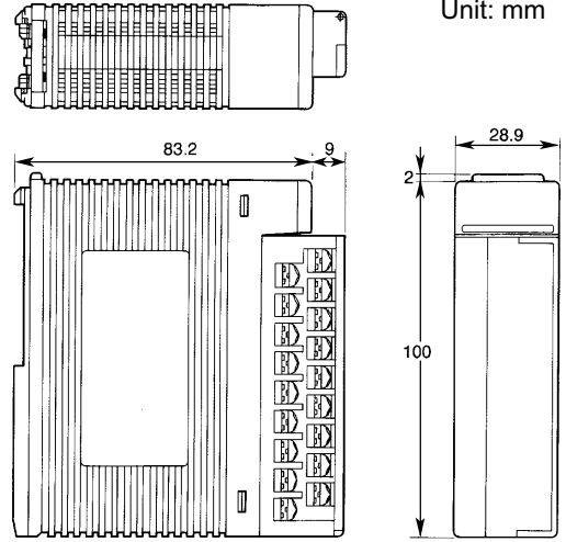
F3YD14, F3YC08-0C, F3YC16
