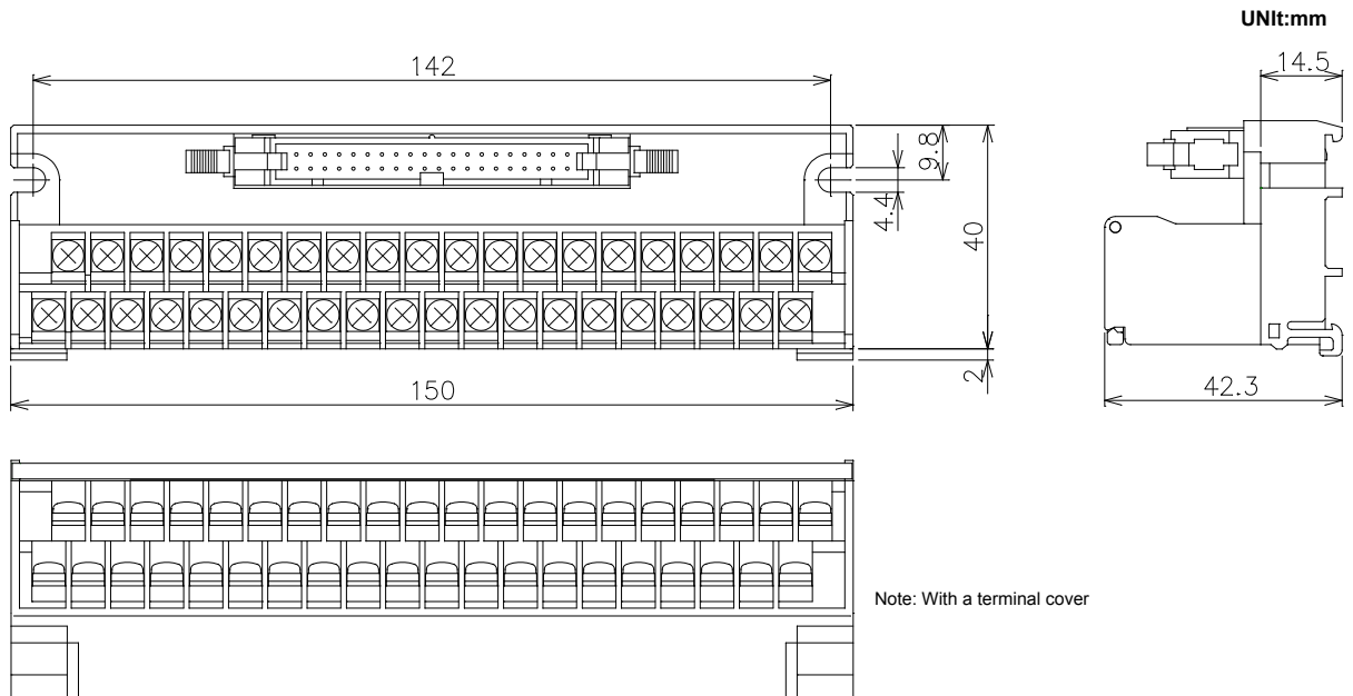
Mounting dimension
